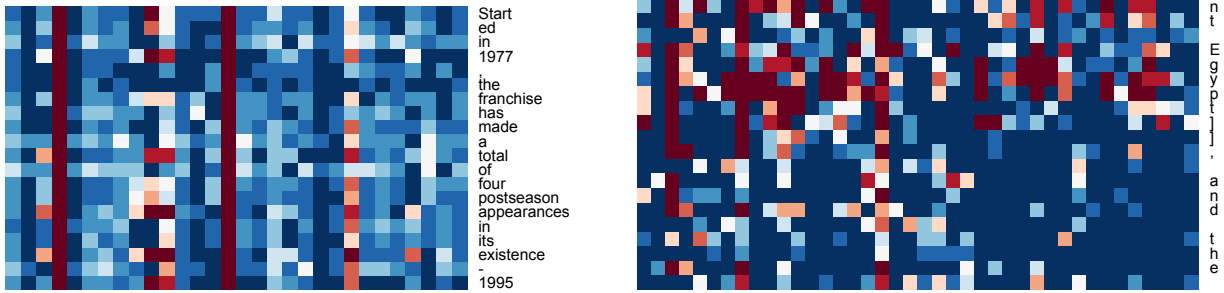
Figure 6: Heatmaps of g values on a partial sequence from WMT development set (left) and enwik8 (right). Each row is a token (word or character), each column is a dimension from g . blue indicates value closer to 1.0, whereas red indicates value closer to 0.0. The darker the shade the closer the value is to the extreme. We see vertical patterns on WMT, indicating that these dimensions are reserved to flow information from long-term memory. Horizontal patterns on enwik8 indicates the model relies on long-term memory to predict a target token (e.g., when forming the word Egypt). The g vector has 512 dimension, we only zoom in to a small dimension subset here. There are more horizontal and vertical patterns on both datasets as a whole.
